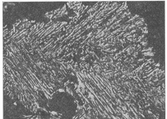
FIG. 2. Pattern of weakness. Type 446 stainless steel, containing 26% chromium and 0.15% carbon, water-quenched from 850° C and embrittled by heating for 200 hrs at 475° C ( \times 850 ).
