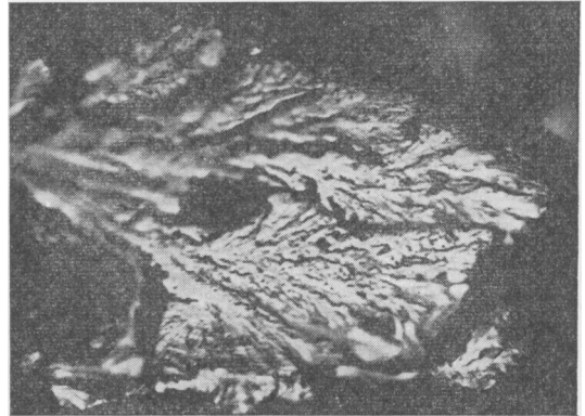
FIG. 1. Pattern of "toughness." A cast steel containing 7.70% chromium and 0.10% carbon, air-cooled from 875° C to produce martensite ( \times 2,000 ).
